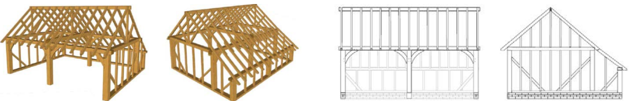
D03 : Three bay or more – cat slide
